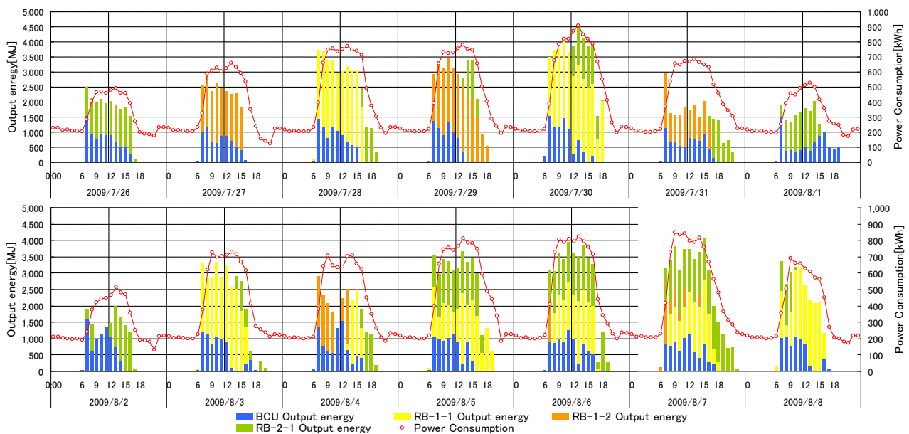
Figure 5. Operation records of cooling source
