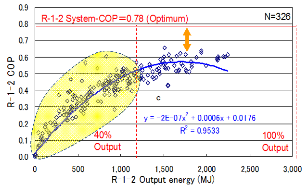
Figure 8. Output and system-COP (R1-2)
