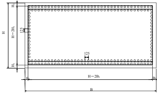
Fig.3 Cross section of a pier
