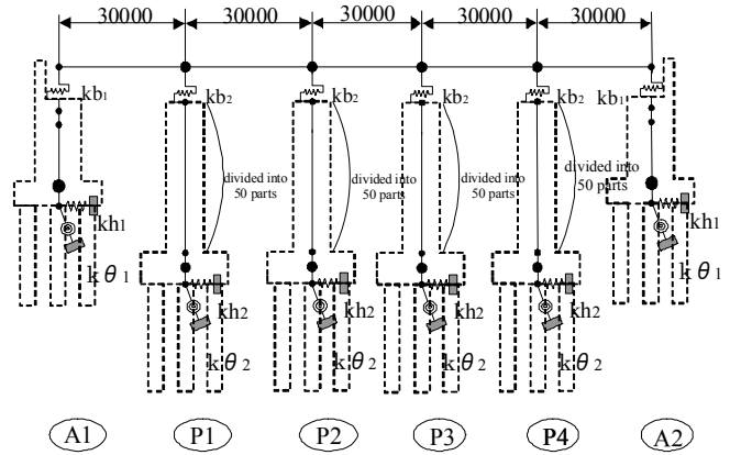
Fig.5 Nonlinear seismic response analysis model
