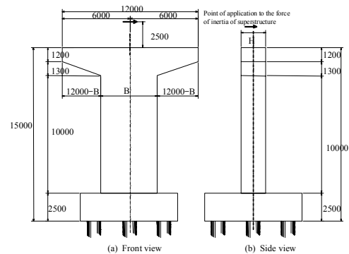
Fig.2 Front and side views of piers and RC pile foundation
