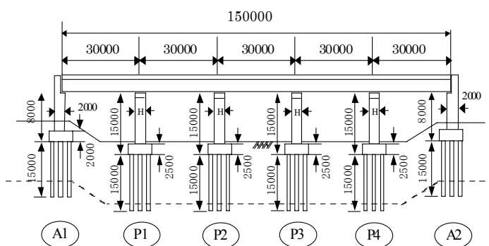
Fig.1 Five-span continuous steel girder bridge system
