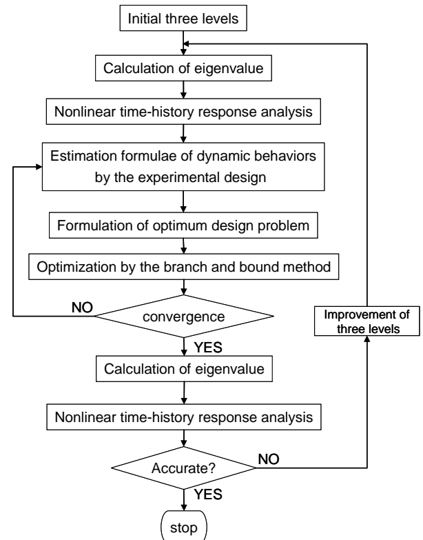
Fig.6 Macro-flow of the proposed optimum design method
