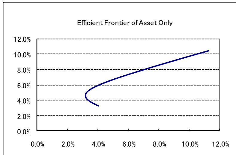
Figure 2-(b). Efficient Frontier of Asset Only ; \sigma = 3.00\%
