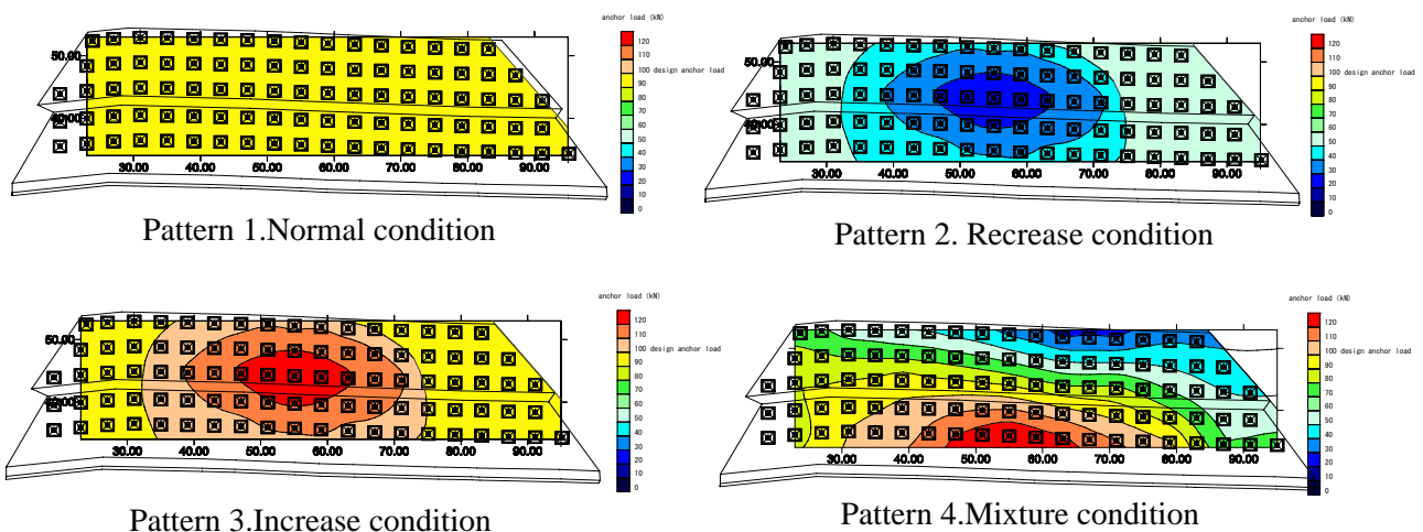
Figure 1. Disutribution pattern of anchor load
