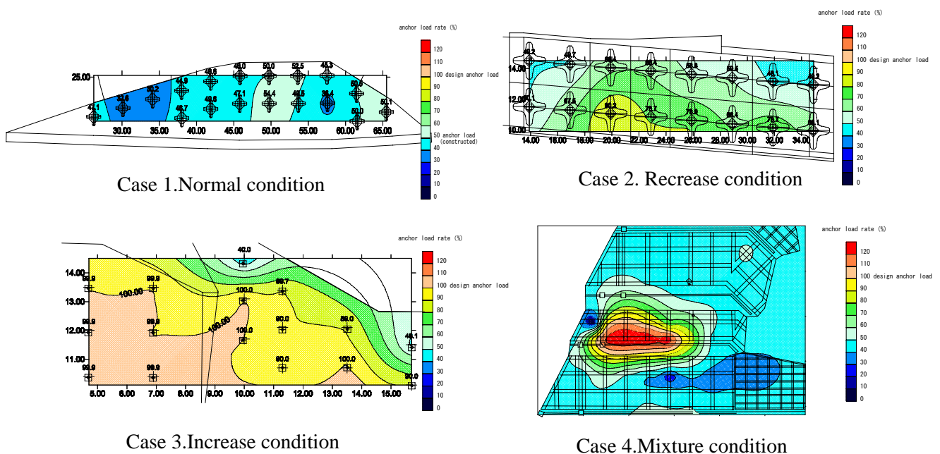
Figure 4. disistribution of anchor load
