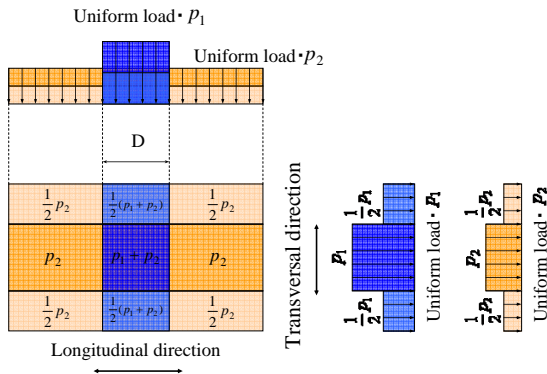
Fig.6 L load
