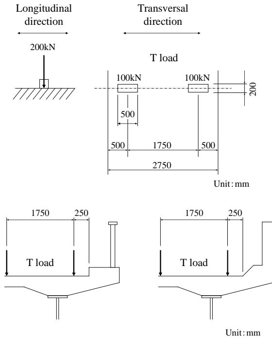
Fig.5 T load
