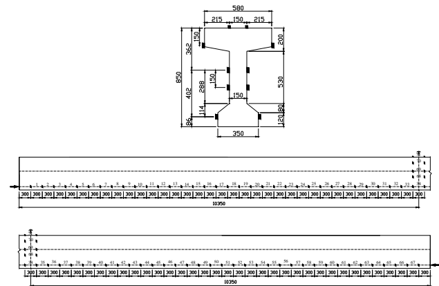
Fig.11 Position of gauge plug and measured camber
