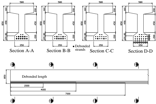
Fig.7 Position of PC strands in section and bond control length
