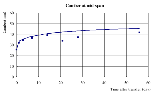
Fig.13 Experiment and calculation result of camber
