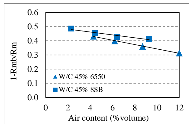
Figure 9. Effect of different type of superplasticizer on 1-R_{mb}/R_m , which W/C 45%
