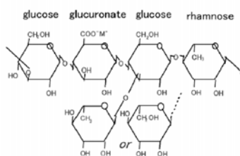
Fig.4. Chemical structure of Welan gum (Sakata et al., 2003)
