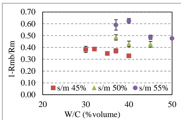
Figure 7. Effect of W/C on 1-R_{mb}/R_m
