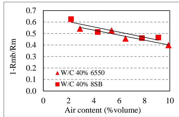
Figure 8. Effect of different type of superplasticizer on 1-R_{mb}/R_m , which W/C 40%
