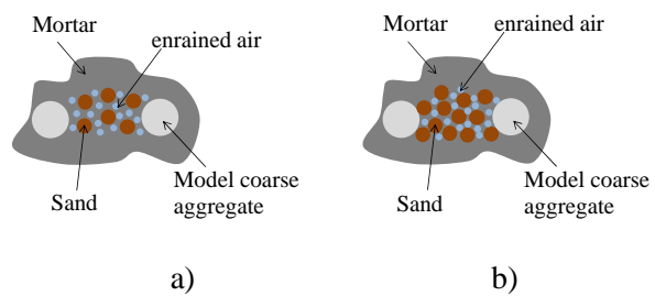
Figure 12. Effect of entrained on distance between model coarse aggregate a) long distance (low s/m), b) short distance (high s/m)
