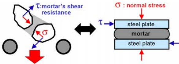
Figure 2. Shear resistance of mortar ( \tau ) in accordance with normal stress ( \sigma ) (Okamura et al., 1993)
