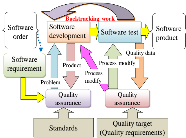
Figure1 Software quality management Model
