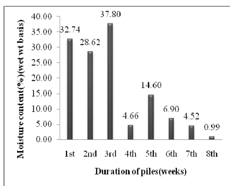
Figure 6 variation of percent moisture content of the composting pile with time
