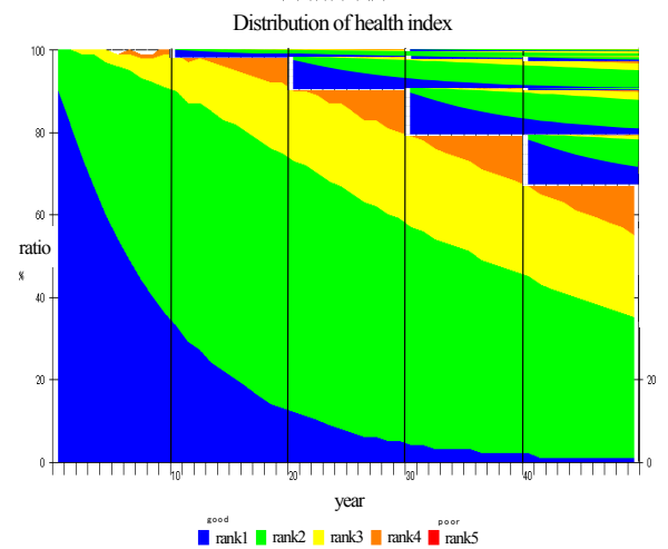
Fig.2 Distribution of health index (repair lower than rank 4 every ten years)
