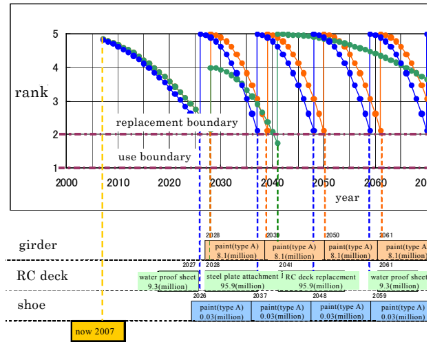
Fig.5 LCC (graph type)
