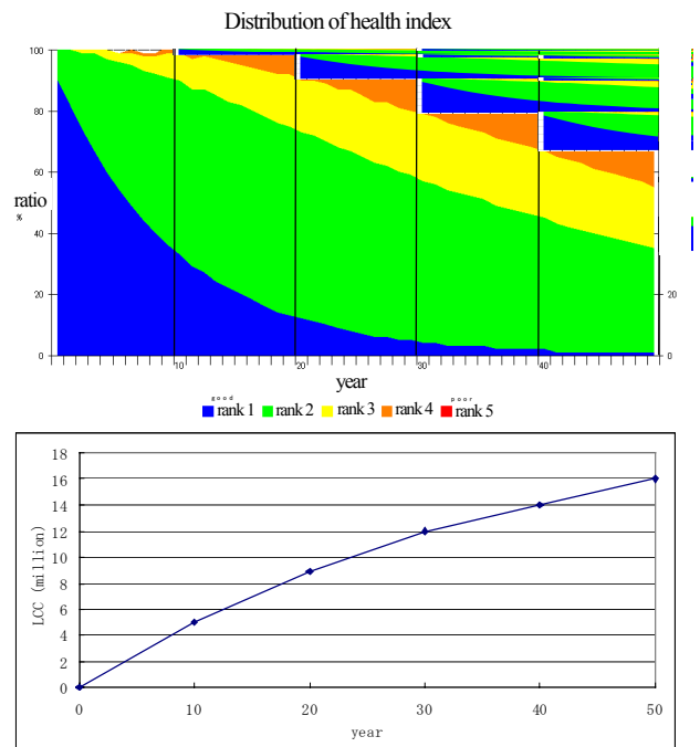
Fig.6 LCC (state transition type, repair lower than rank 4 every ten years)
