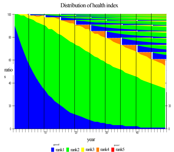
Fig.1 Distribution of health index (repair lower than rank 4 every five years)
