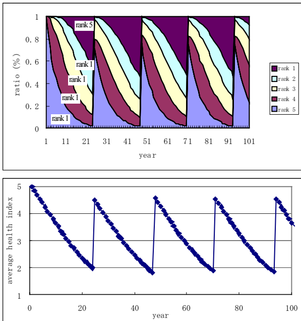
Fig.12 Transition of state distribution and average health index (p=0.85, considering state distribution, repair on average rank 2)
