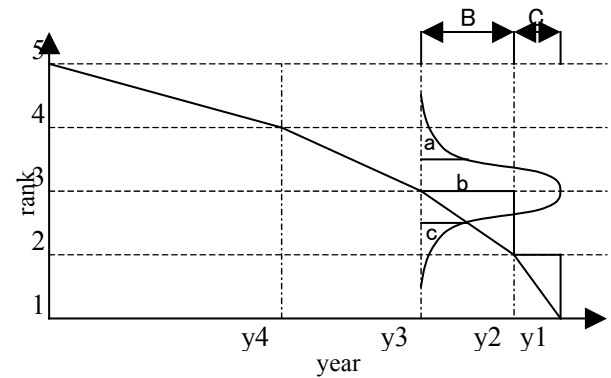
Fig.4 Image of state distribution on deterioration curve of graph type
