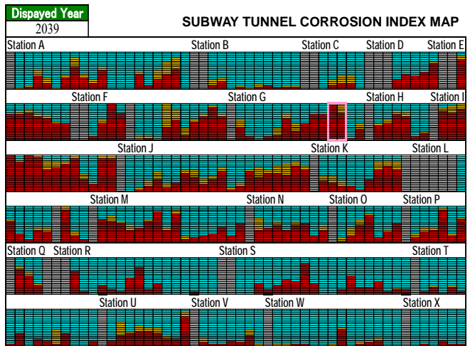
Figure 3.5 Corrosion index map 30 years later
