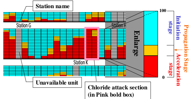
Figure 3.6 Description of corrosion index map
