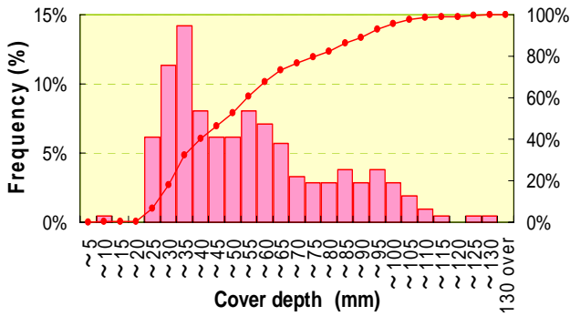
Figure 3.2 Measured cover depth in a control unit
