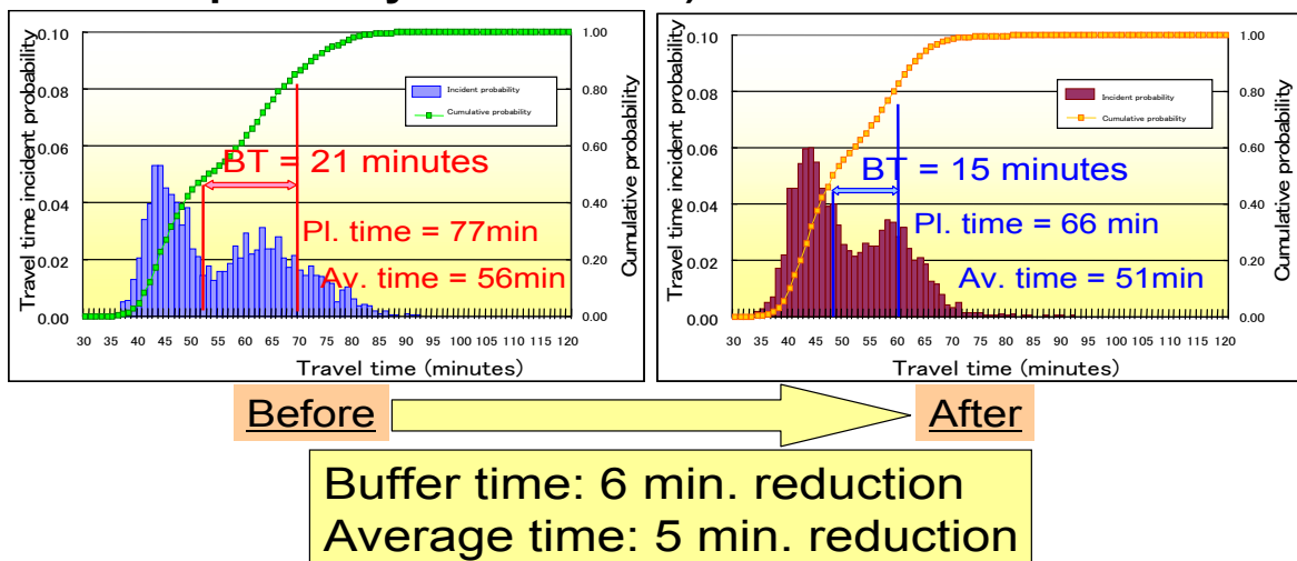
Figure 3.3.2.2 Travel Time Reliability
