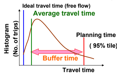
Figure 3.3.5 Reliability of Travel Time using Bus-Location Data
