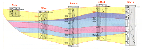
Fig.2 Stratum profile
