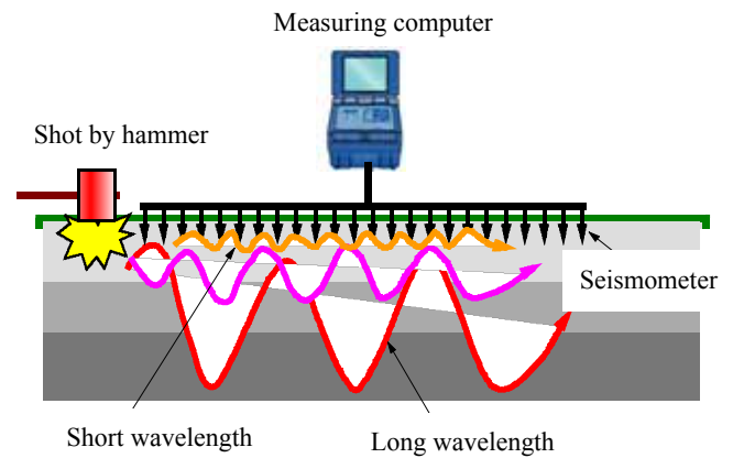
Fig. 1 Surface wave prospecting
