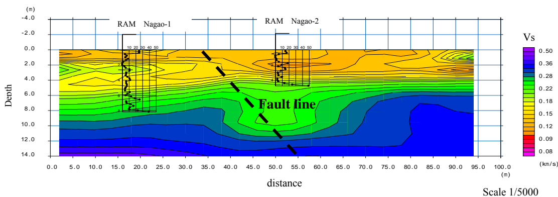
Fig. 4 S-wave velocity contour at Tanaka site
