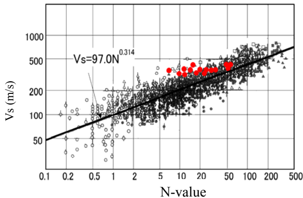
Fig. 8 Relation between N-value and Vs (Imai et al,1982)
