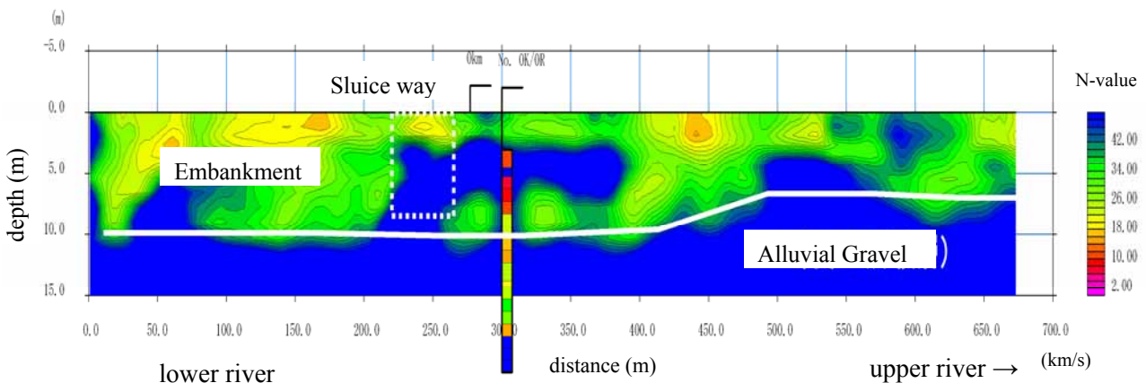
Fig. 9 Estimated N-value contour
