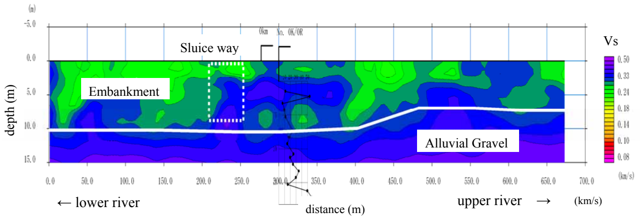
Fig. 7 S-wave velocity contour
