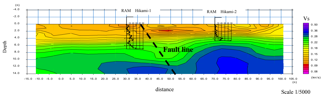
Fig.5 S-wave velocity contour at Hikami-Miyashita site
