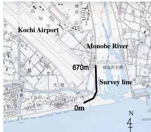
Fig.6 Location of survey(mouth of Monobe River)
